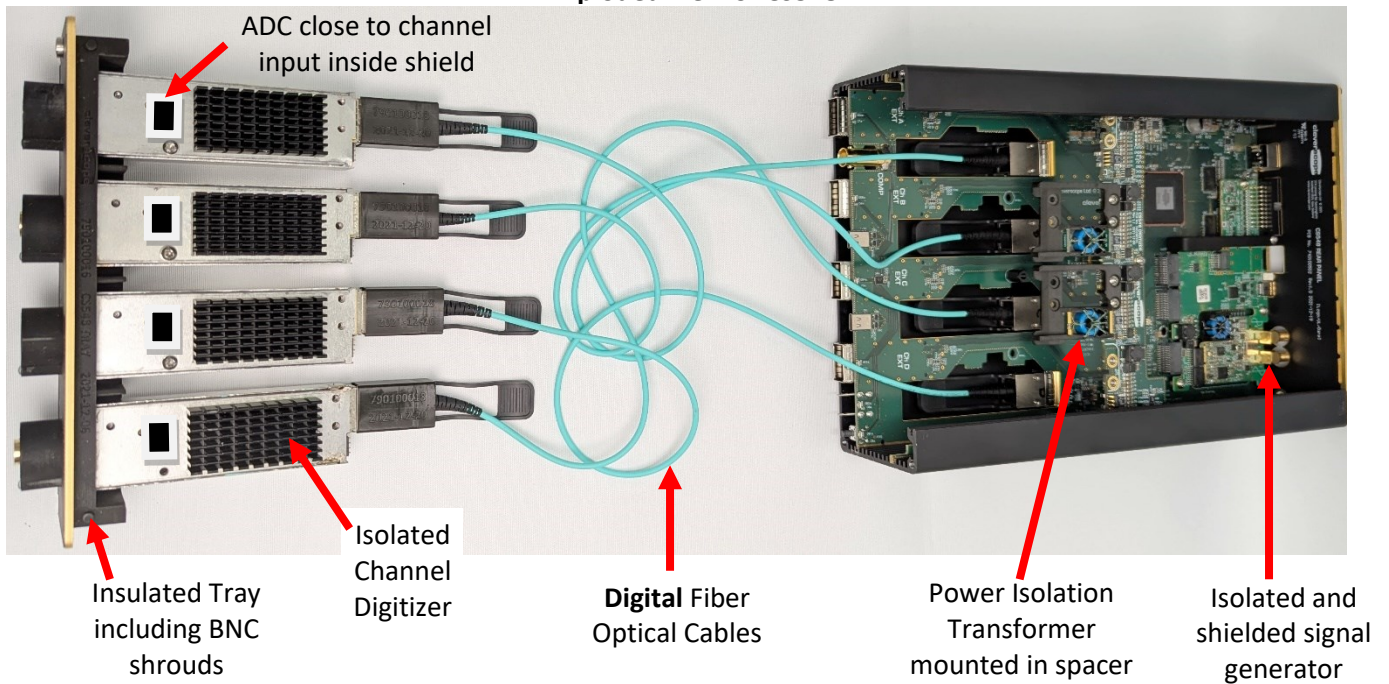
Exploded view of CS548
